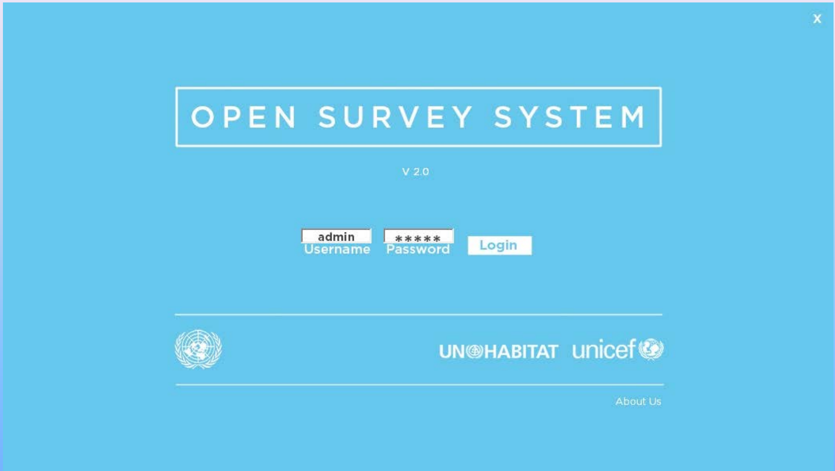
Figure 1. Login Form
