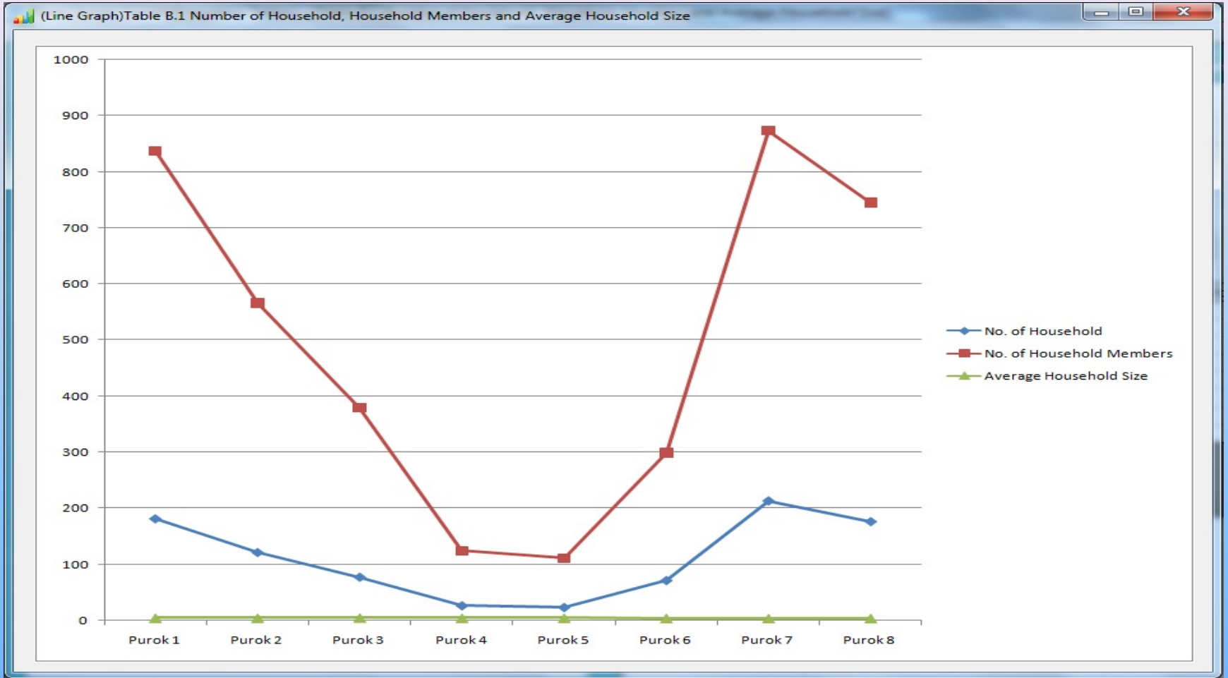
Figure 6. Generate Graph
